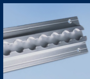
07 alu lashing track, can be countersunk in Soboflex safety floor
